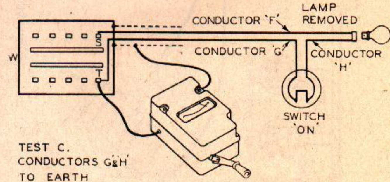
Figure 14 Test to locate fault to earth on branch circuit
