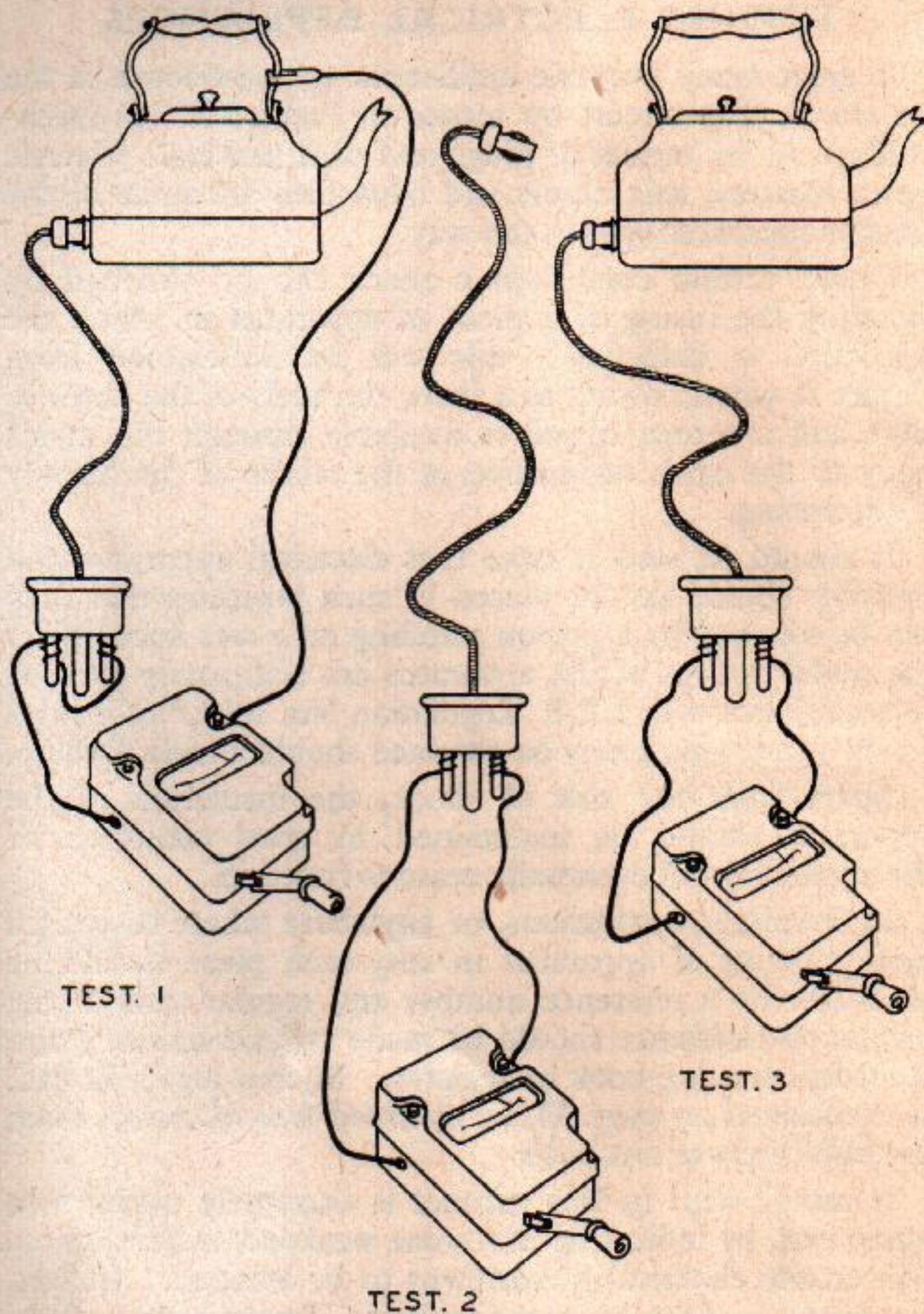
Figure 4. Tests on an electric kettle
