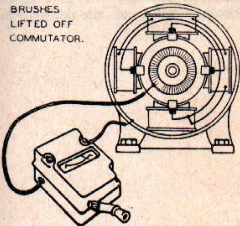
Figure 9 Test on armature only.
